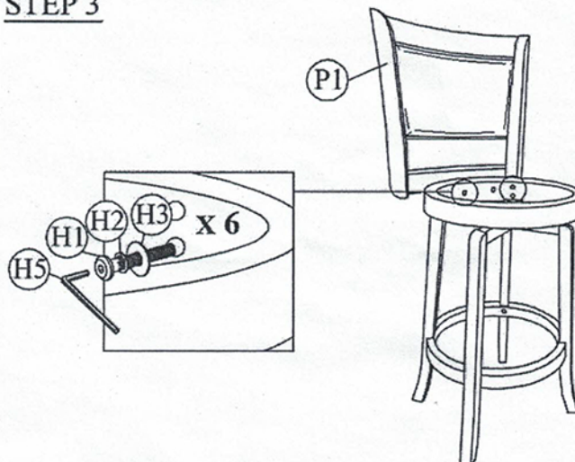
COMPLETE ASSEMBLY
